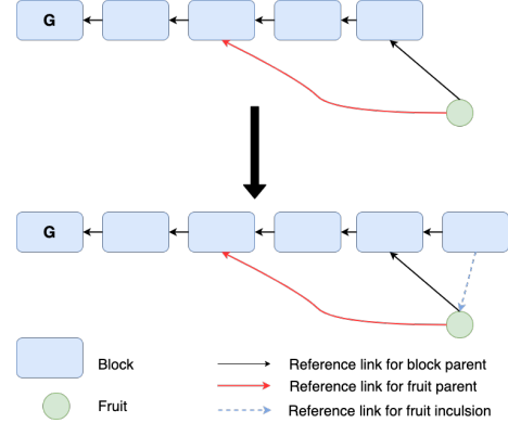
Figure 8: The FruitChains protocol.
