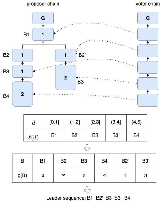
Figure 5: An example of the ledger formation rule in Prism. For simplicity, we only have one voter chain in the example. The number inside each proposer block is the block difficulty. In this example, the heaviest proposer chain has chain difficulty 5. We find the leader block \ell(d) for each difficulty level d in (0, 5] according to the votes (as shown in the first table). Then we find the grade g(\cdot) of each proposer block by Equation (1) as shown in the second table. Finally, the proposer blocks are ordered by their grades.
