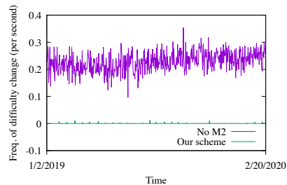
Figure 13: Frequency of difficulty change on a non-pivot chain where 30% of miner power is adversarial.
