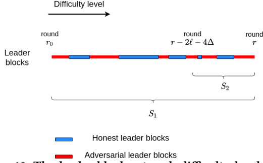
Figure 10: The leader blocks at each difficulty level in the proposer tree.
