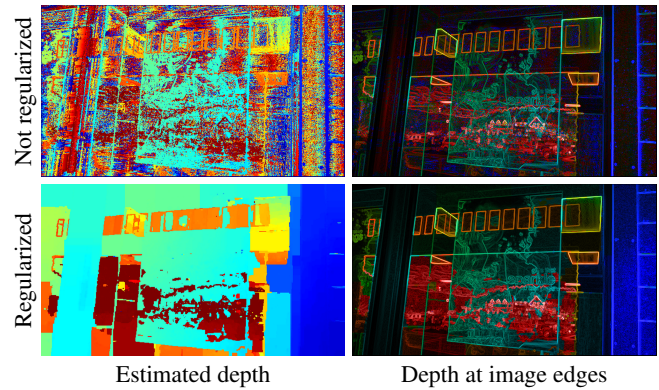
Figure 3: Stereo reconstruction, unregularized (top) and regularized (bottom). In the right column we modulated the depth maps by gradient magnitude to visualize that the depth is correct at image edges. Regularization produces more consistent results, while still being correct at strong gradients.
