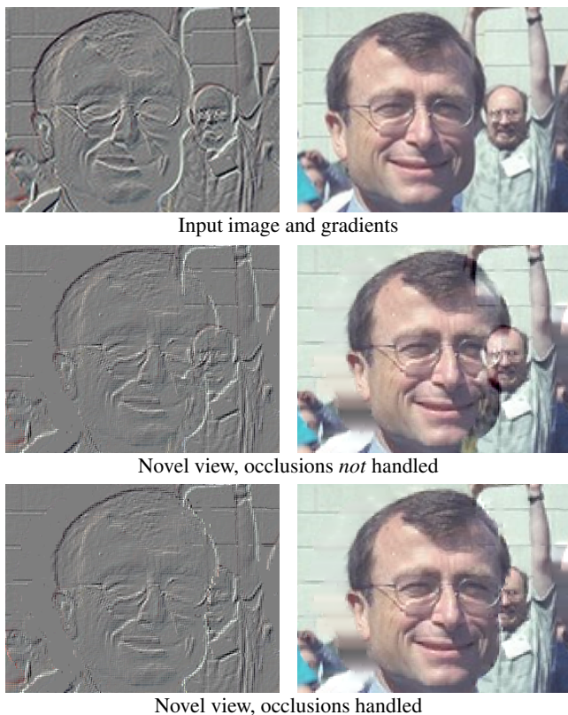
Figure 7: Oclusions and disocclusions. Note how the disocclusions to the left of the neck are smoothly filled in by the Poisson integration.
