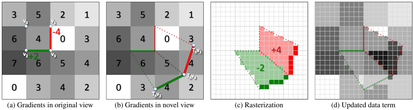
Figure 5: Computing the approximate solution in the general case. Each gradient (a) generates a quad connecting its locations in the original and novel view (b). The quad is rasterized (c) and splatted with additive blending updating the underlying image (d). In Figures (c) and (d), the small pixels can also be thought of as the super-samples used in anti-aliasing. The dark red and green lines in (c) are the spine of the 1-pixel wide anti-aliased lines used to splat the gradients into the gradient buffer.
