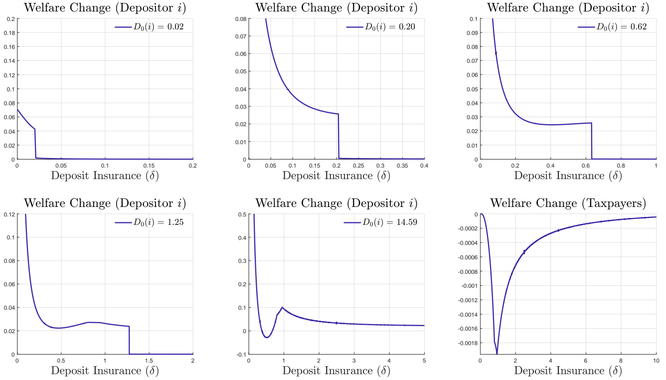
Figure 9: Distributional Considerations
