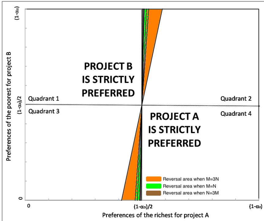
Figure C2. \theta = -0.5 (complementarity)
